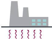
Geothermal energy
